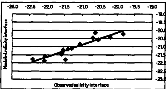
Fig. 8 Comparison of observed and modeled interface at well # 1
