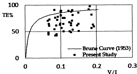
Figure 11 - Comparison of experimental results with the Brune curve [4]
