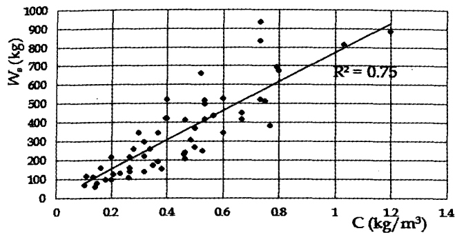
Figure 10 - Variation of C versus W_s
