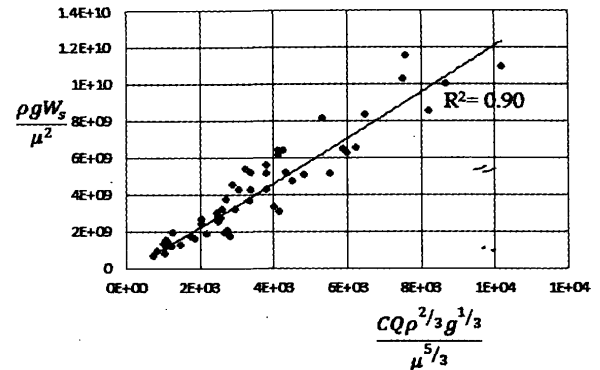
Figure 14 -Variation of non-dimensional terms representing W_s and CQ
