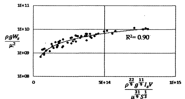
Figure 15 -Variation of trapped sediment weight ( W_s ) with the model parameters
