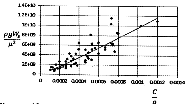
Figure 13 - Variation of non-dimensional terms representing W_s and C
