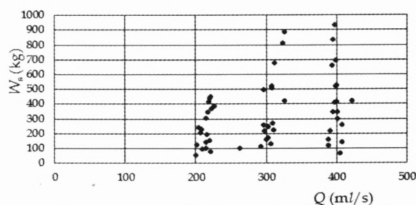
Figure 9 - Variation of Q versus W_s
