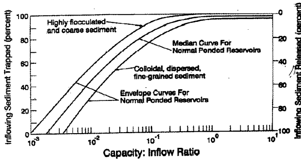
Figure 1 -Brune curve [4]
