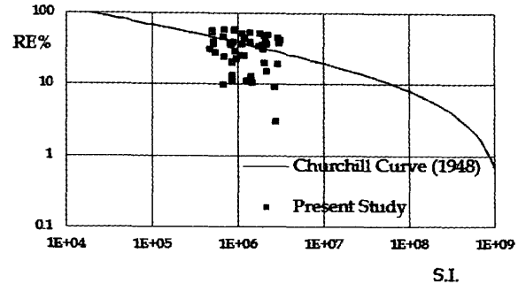
Figure 12 -Comparison of the experimental results with Churchill curve [5]
