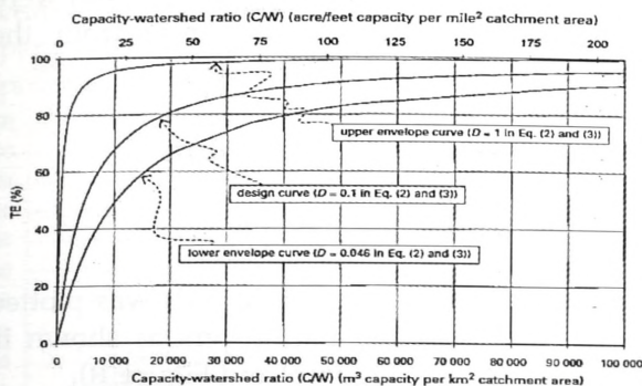
Figure 3 - Brown's curve [3]
