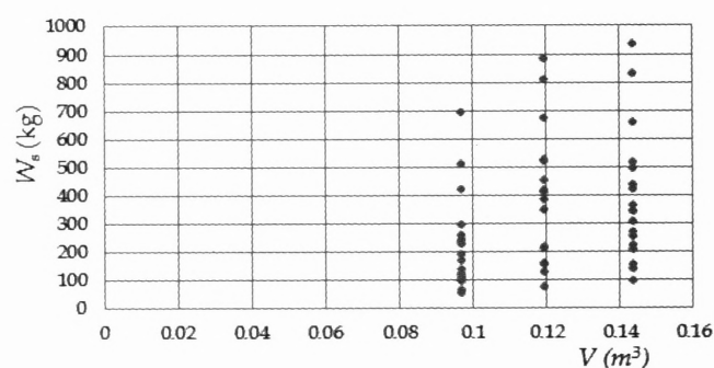
Figure 8 - Variation of V versus W_s
