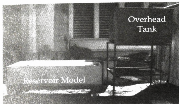
Figure 5 -Experimental Set-up
