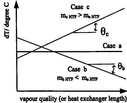
Fig. 3 : Degree of temperature glide match (relative to the cold end) [9]
