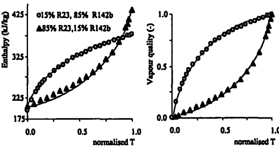
Fig. 6 : Two-phase non-linearity of refrigerant mixture [2]
