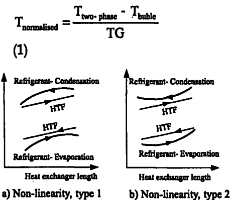
Fig. 5 : Effect of property non-linearity on glide matching
