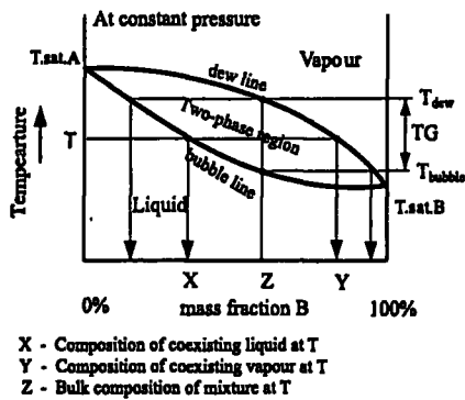
Fig. 1 : Phase changing process of a binary mixture
