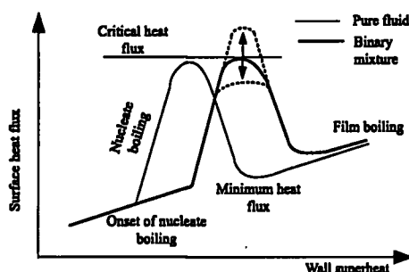
Fig. 7 : Principal changes to boiling curve for a binary mixture [24]
