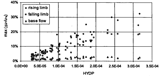
Figure 6: Variation of maximum (\Delta u./u_{*s}) with HYDP in the rising branch (accelerating flow) and falling branch (decelerating flow) of the hydrographs.
