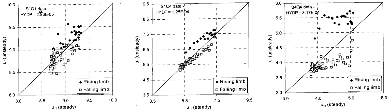
Figure 3: Comparison of shear velocities computed by steady and unsteady state formula during the passage of a hydrograph
