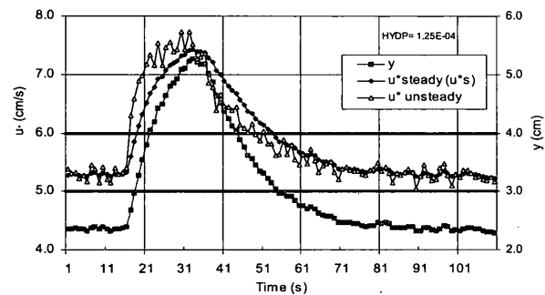
Figure 2: Variation of water depth and shear velocity in an unsteady flow run.
