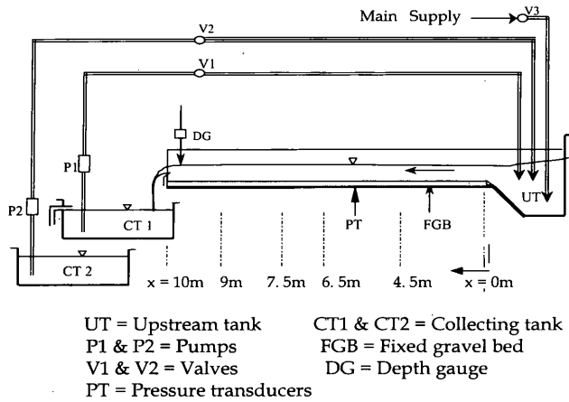
Figure 1: Experimental set-up
