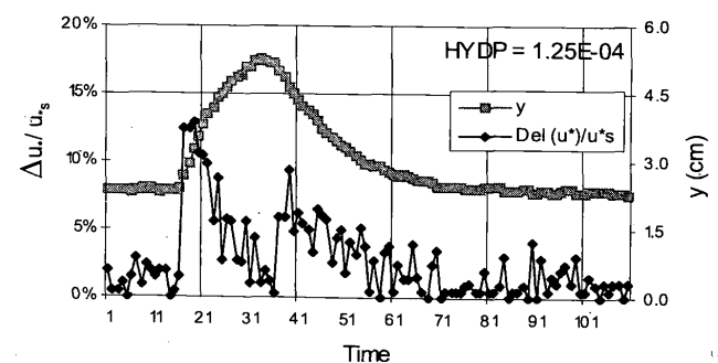
Figure 5: A typical plot of time variation of \Delta u^* / u^*_s during the passage of a hydrograph.
