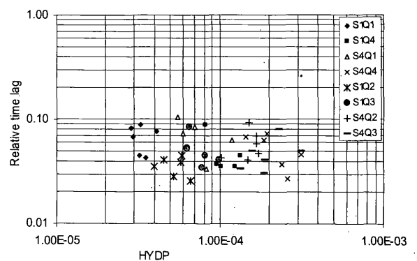
Figure 4: Relative time lag Vs hydrograph parameter
