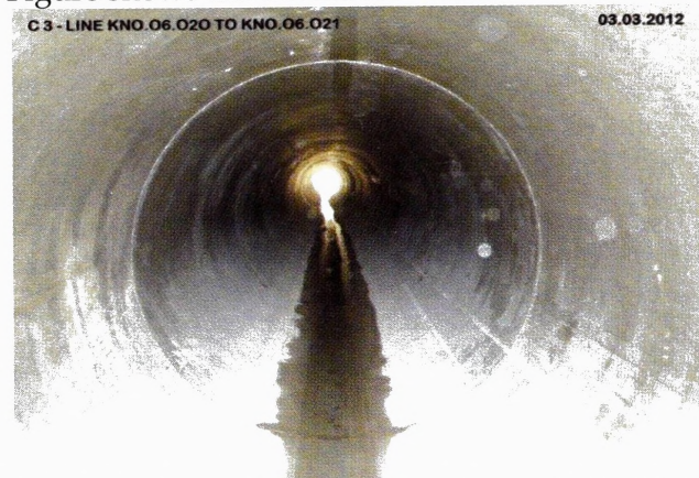
Figure 3 - Deviation of pipeline at AlKhuwair
