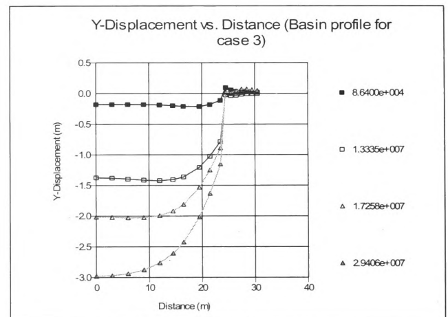
Figure 8: Basin analysis (settlement of the embankment) for case 3
