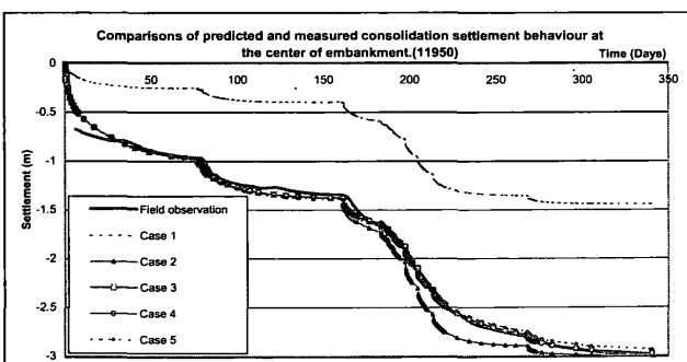
Figure 3: Comparison of the consolidation settlement at 11950 at centre of the embankment.
