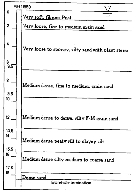
Figure 1: Profile of subsurface conditions across 11950 location
