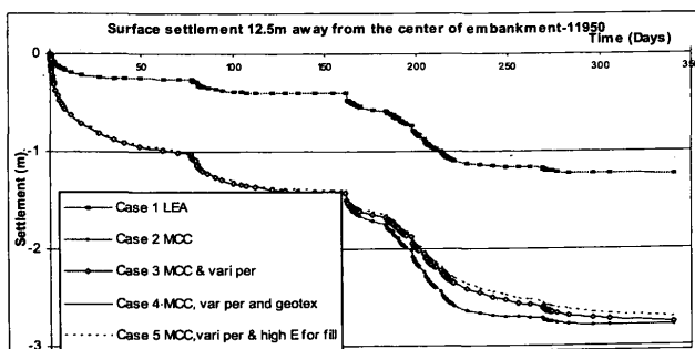
Figure 4: Predicted settlement at 11950 at 12.5m away from the centre of embankment.
