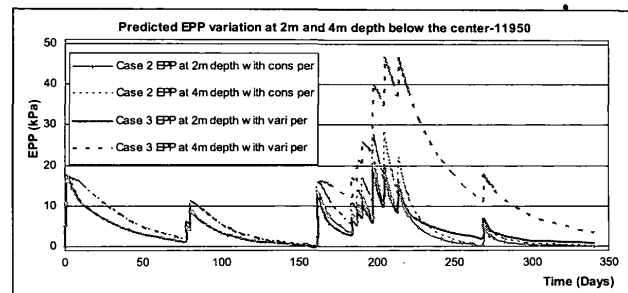
Figure 5: Predicted EPP at 2.0m and 4.0m depth at the centre of embankment
