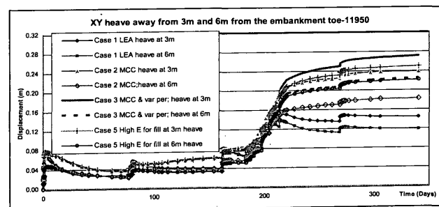
Figure 6: XY (resultant) deformation patterns away from embankment toe.
