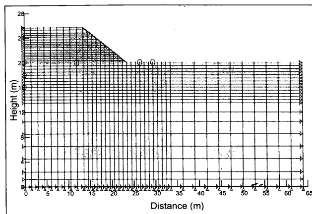
Figure 2: Finite element mesh for 11950 section
