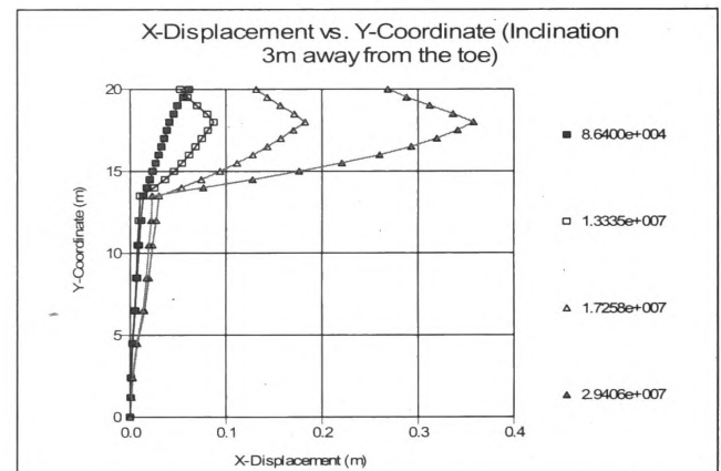
Figure 9: Prediction of horizontal displacements 3.0m away from the toe for case 3
