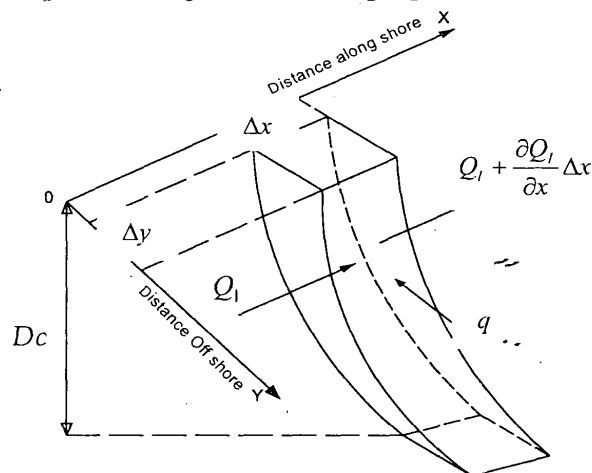
Figure 1 - Sketch of sediment balance
