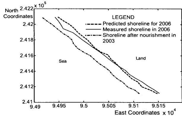
Figure 4 – Comparison between the simulated and measured shoreline positions in 2006 obtained during model calibration.
