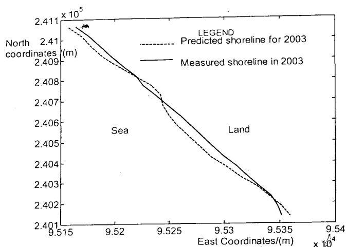
Figure 6 - Comparison of the measured shoreline position before sand nourishment in 2003 with the predicted shoreline after 4 years.
