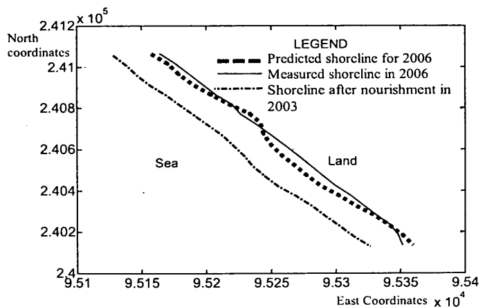
Figure 5 – Comparison between the simulated and measured shoreline positions in 2006 obtained during model verification.
