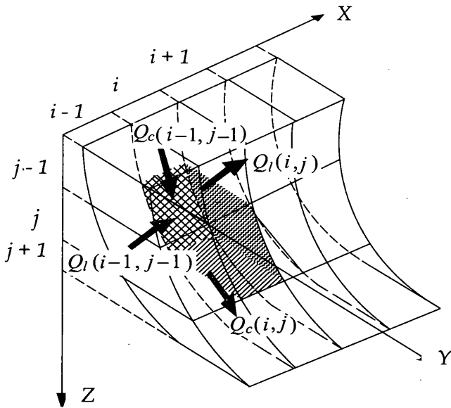
Figure 2 – Sediment entering and leaving a given element in N- Line model
