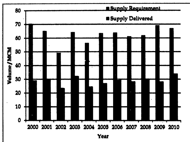
Figure 12 -Comparison of Supply Requirement and Supply Delivered in LB Area
