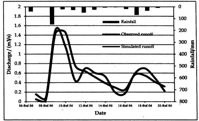
Figure 7- Validation of Event Based Simulation
