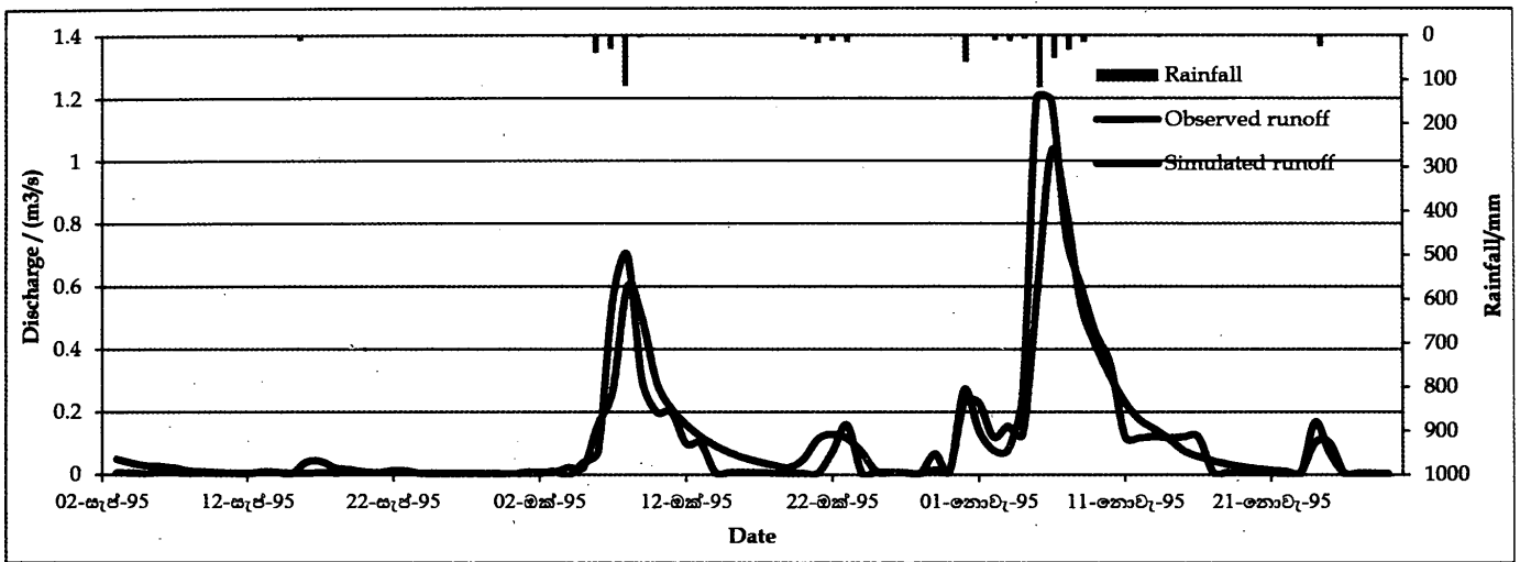
Figure 8 - Calibration of Continuous Simulation
