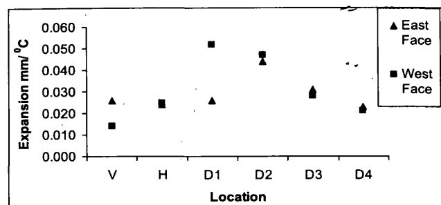
Figure 10 - Average maximum daily expansion of the 2 m concrete framed wall model (Model III)
