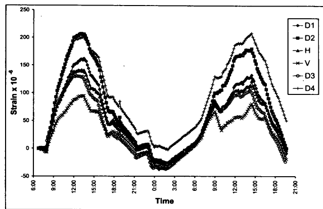
Figure 11 - Strain measurements in 2 m load bearing wall model - West Face
