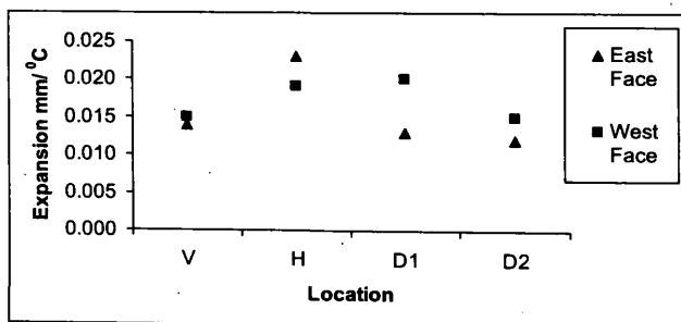
Figure 8 - Average maximum daily expansion of the 1 m load bearing wall (Model I)
