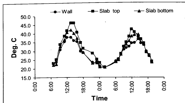
Figure 3 - Temperature variation of 2 m load bearing wall model
