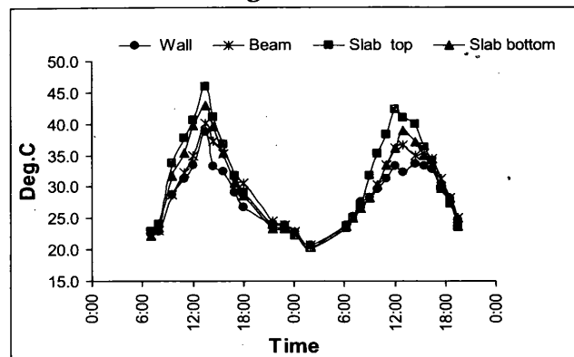
Figure 3 - Temperature variation of 2 m load bearing wall model
