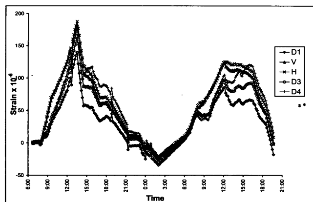
Figure 12 - Strain measurements in 2 m concrete framed wall model - East Face
