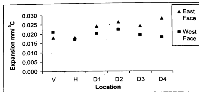
Figure 9 - Average maximum daily expansion of the 2 m load bearing wall model (Model II)
