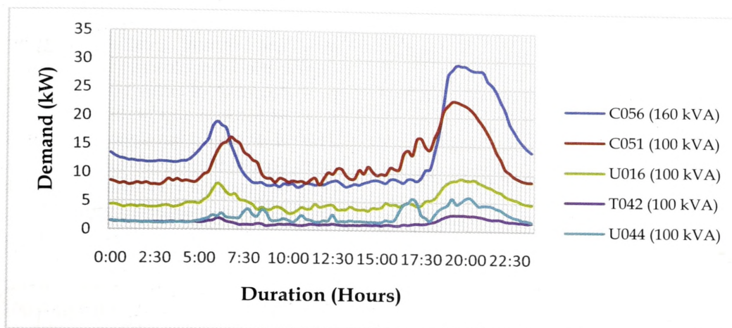
Figure 1 - Demand Curves for Distribution Transformers in Rural Areas
