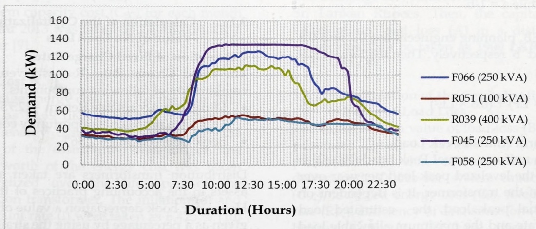
Figure 3 - Demand Curves for Distribution Transformers in Urban Areas
