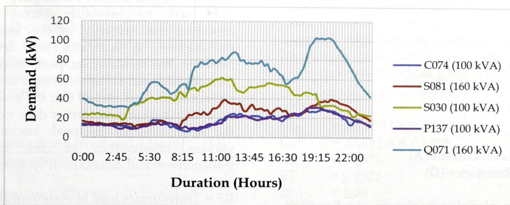
Figure 2 - Demand Curves for Distribution Transformers in Semi-urban Areas
