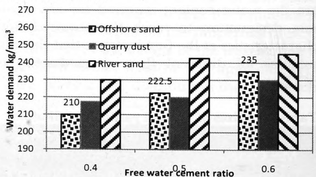
Figure 10 - Water demand by different aggregate types at different w/c ratio at 70% fine aggregate proportion
