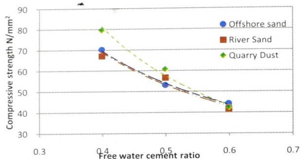
Figure 13 - Average strength vs. water cement ratio for SCC
