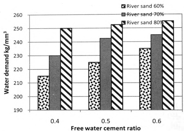
Figure 9 - water demand with the increasing water/cement ratio
