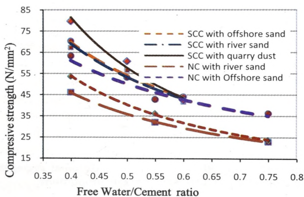
Figure 15 - Strength vs. w/c ratio for the three aggregate types for normal and self-compacting concrete.
