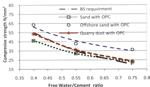
Figure 14 - Average strength vs. water cement ratio for Normal Concrete
