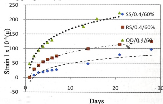
Figure 16- Typical shrinkage measurement of SCC for various aggregate types
