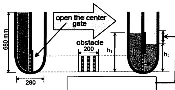
Figure 4(a) - U box test: Difference in the two legs is taken as a measure of the flow ability (passing ability) of the concrete mix
