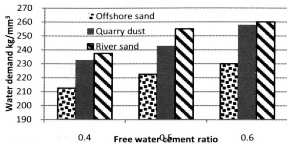
Figure 11- Water demand for different aggregate types with common particle size distribution operated at 70% of fine aggregate proportion
