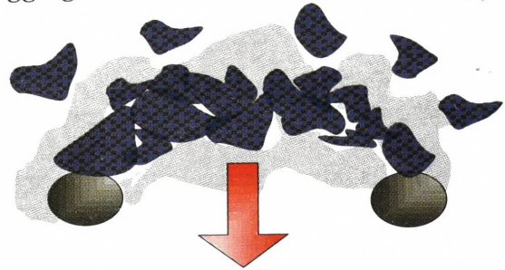
Figure 2(b) - Aggregate arch blocking the passing ability in SCC
