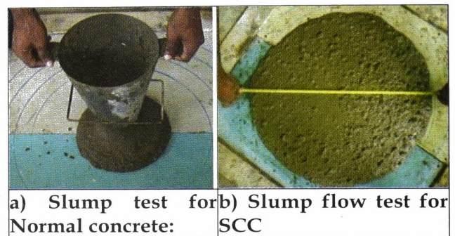
Figure 3 - Measure of flow ability (filling ability) of the SCC mixes.
