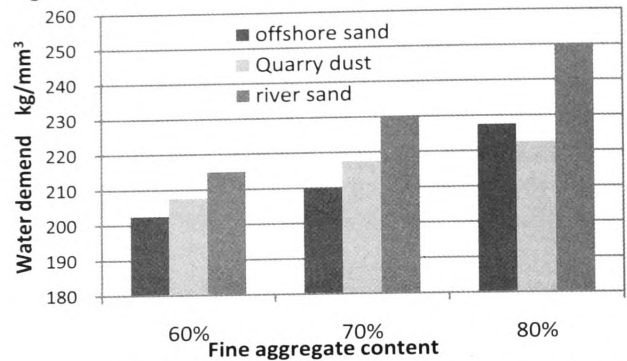
Figure 8 - Increase in water demand with the increase in aggregate proportions recorded for W/C ratio of 0.4.
