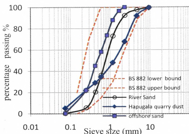
Figure 6 - Particle size distribution of different fine aggregate types compared with the upper and lower bounds of the BS882 requirement for concrete.
