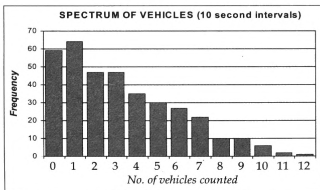
Figure 2 - Spectrum of vehicles at 10 second intervals
