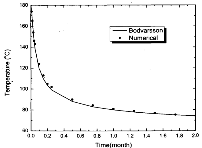
Figure 4-Comparison of the Bodvarsson solution and a numerical solution
