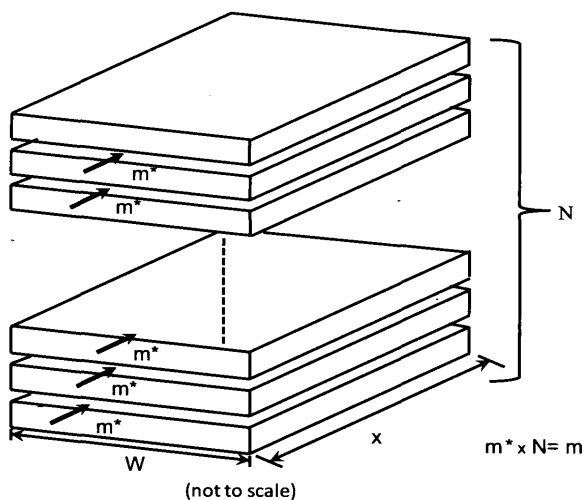
Figure 2 - Illustration of different geometrical variables and the flow rate in Bodvarsson's equation
