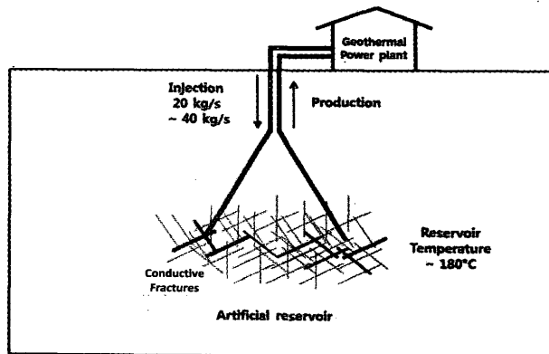
Figure 1 - Conceptual diagram showing a typical enhance geothermal system (EGS)
