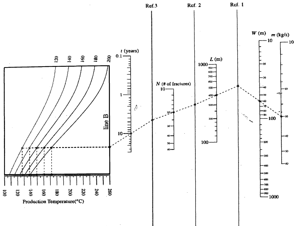
Figure 3- Nomogram for analyzing convection/conductive, coupled geothermal wells (The selected example shows the production temperature after 10 years)
