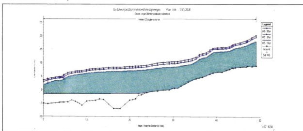
Figure 5.3.1 water surface profiles for 10year, 20 year and 50 year return periods
