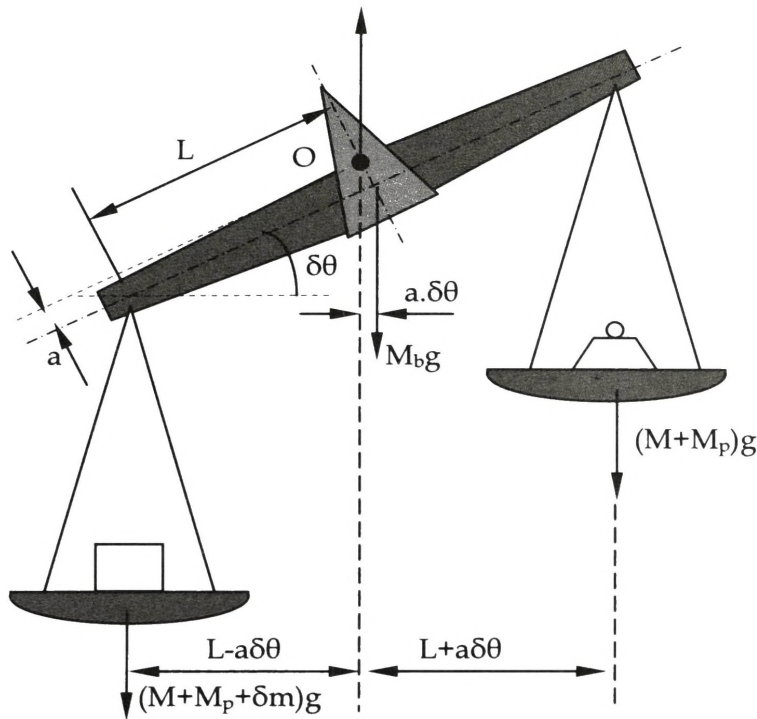
Fig. 2 Operating Principle of an Equal Arm Balance
