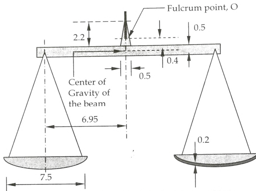
Fig 3 Hypothetical dimensions of balance
