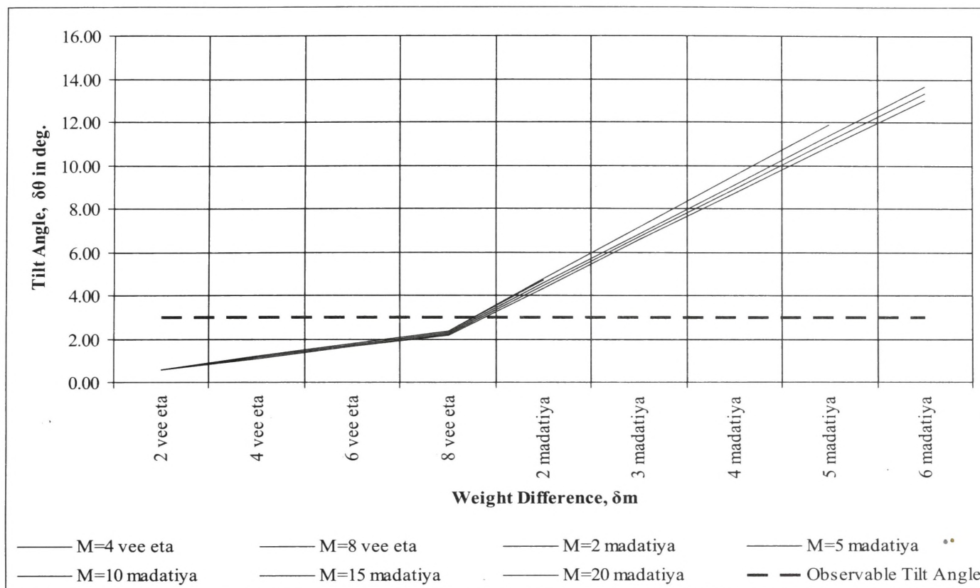
Fig 4 Tilt angle for Weight differences
