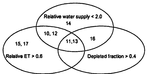
Fig. 3: Venn diagram for the upper range of the performance shown by indicators in figure 2
