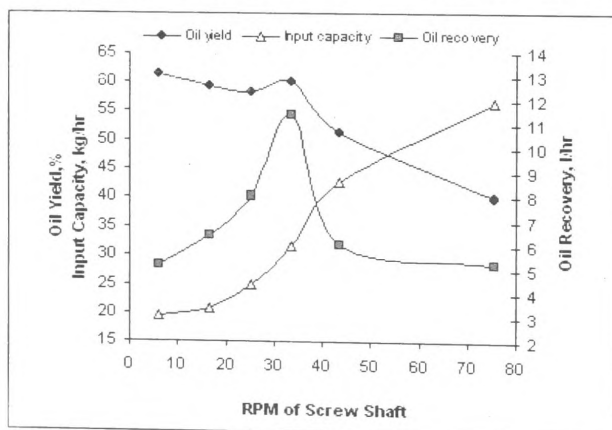
Figure 4. Relationship between RPM of screw shaft with oil yield, input capacity and oil yield
