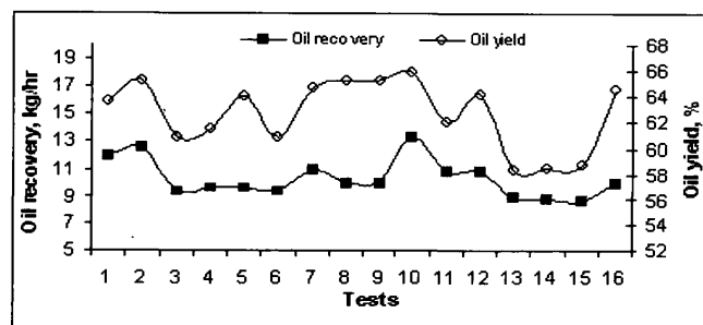
Figure 6. Oil yield and oil recovery of the expeller at field evaluation
