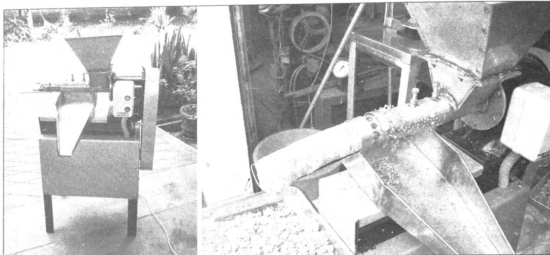
Figure 3. View of the segmented-screw type oil expeller
