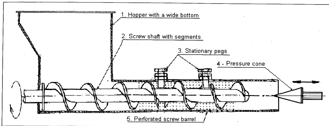
Figure 2. Conceptual design of the screw type virgin coconut oil expeller
