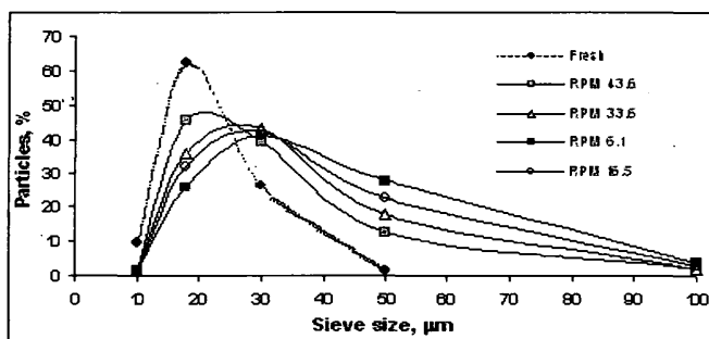
Figure 5. Sieve analysis of input coconut and press cake after oil extraction
