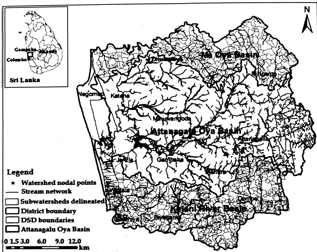
Figure 4 -Attanagalu Oya Watershed and Stream Network
