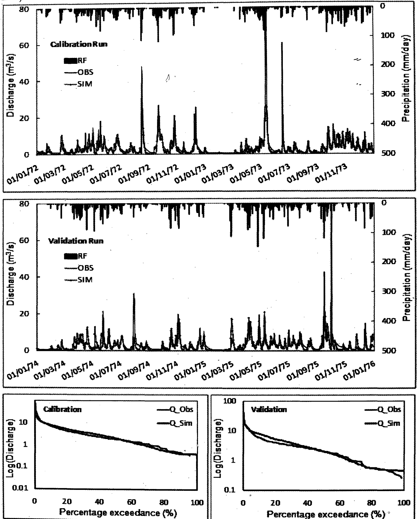
Figure 3 - Comparison of Model Calibration and Verification; a). Calibration run b). Validation run; Flow duration curves for c). Calibration run d). Validation run
