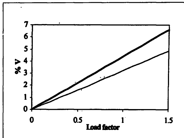
Figure 4.1 - Percentage Voltage Regulation at 0.8 p.f.
