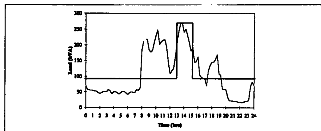
Figure 3.3: Daily Load Profile of Industrial Load
