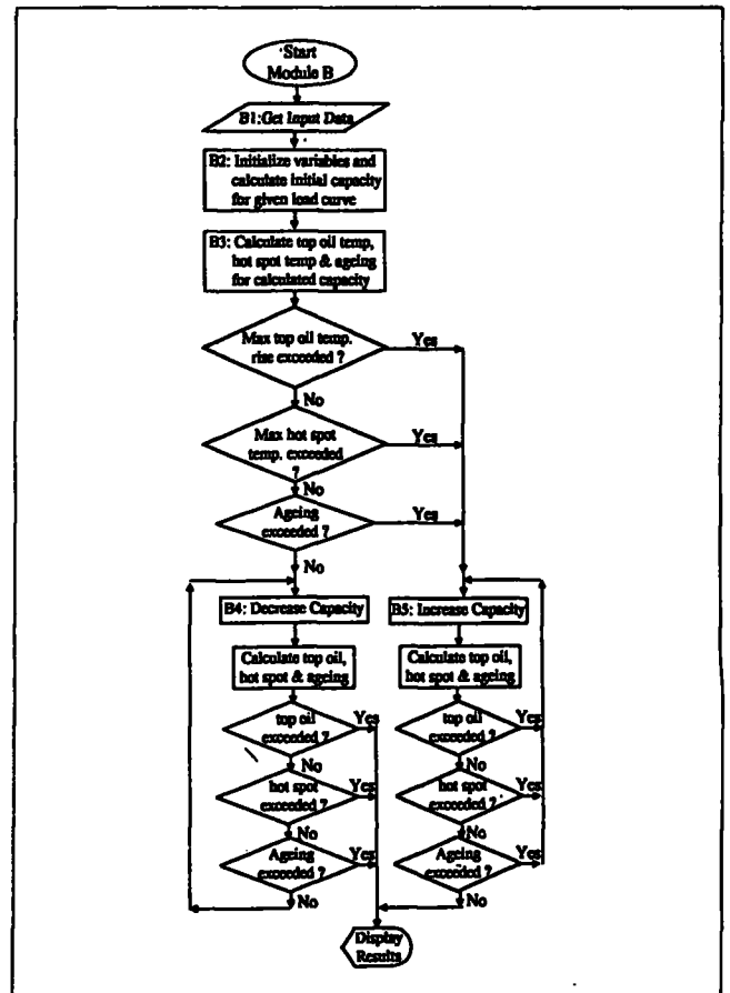
Figure 2.2: Flow Chart for finding Optimum Transformer Capacity
