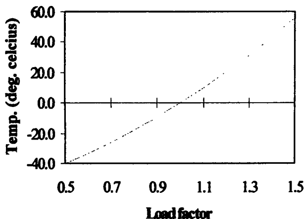
Figure 3.1: Excess in Hotspot temperature with load factor
