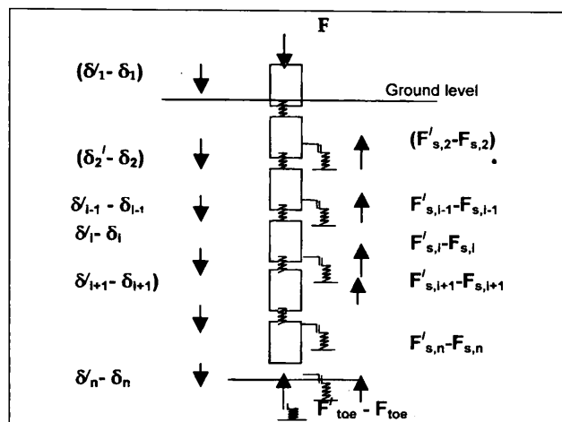
Figure 5: Discretization of the pile with deflection and forces acting on each element.
