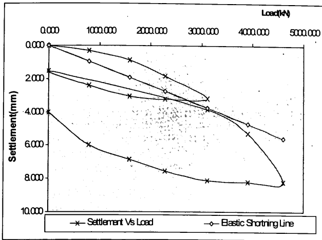
Figure 2: Category I - Initial portion of the Load-settlement curve is above the ELS
