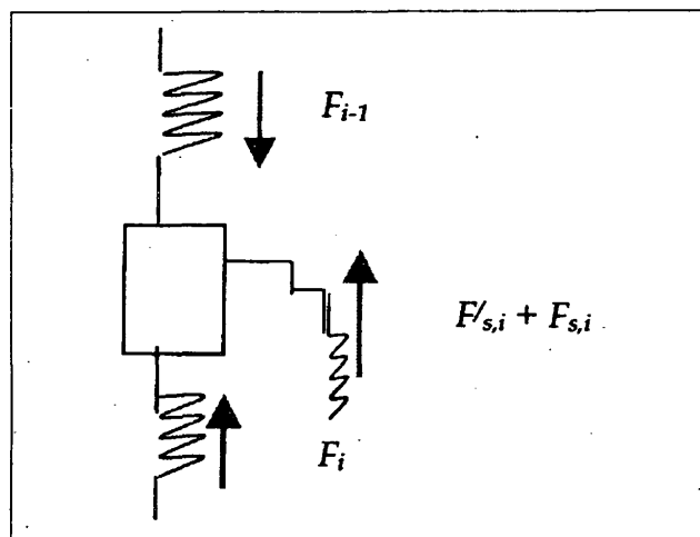
Figure 7: Forces acting on the i^{th} element
