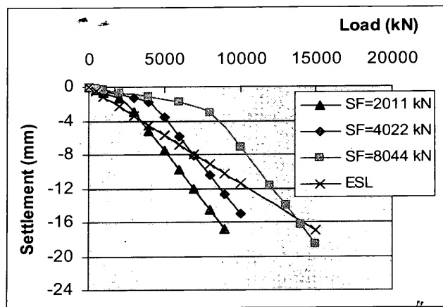
Figure 12: Variation of the load-settlement curve with the SF.
