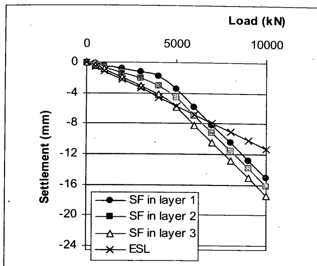
Figure 9: Effect of the location of the SF on the load-settlement curve (End quake 8mm)
