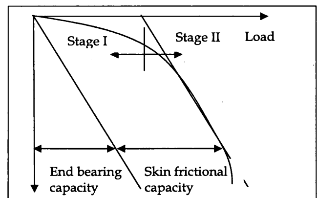
Figure 13: Estimation of the SF and end bearing capacities (Van Weele [8])
