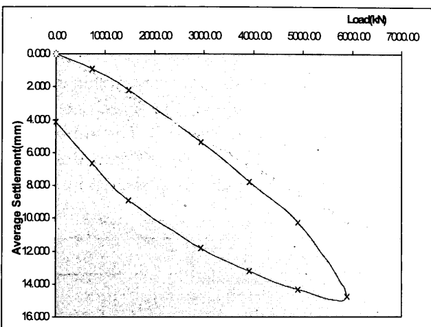
Figure 3: Category II - Initial portion of the load-settlement curve is parallel to the ESL
