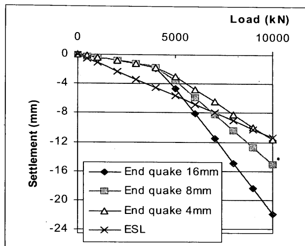
Figure 11: Effects of the changing the stiffness of the end bearing layer on the load-settlement curve.
