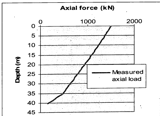
Figure 17: Measured axial force along the pile shaft (Hussein and Camp[2])
