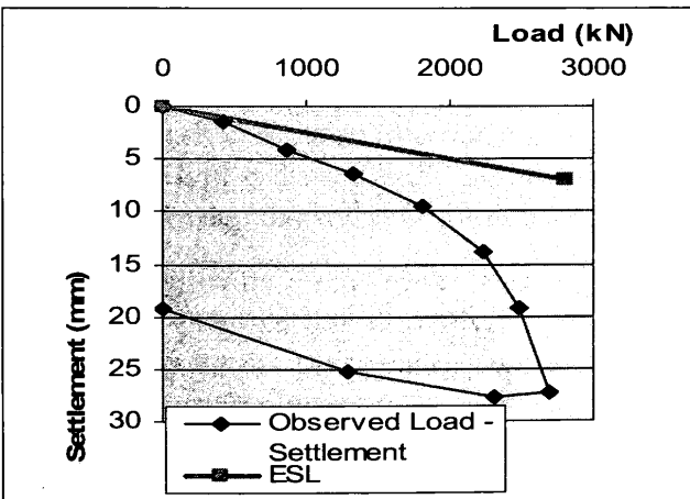
Figure 14: Load -settlement curve (Hussein and Camp [2])
