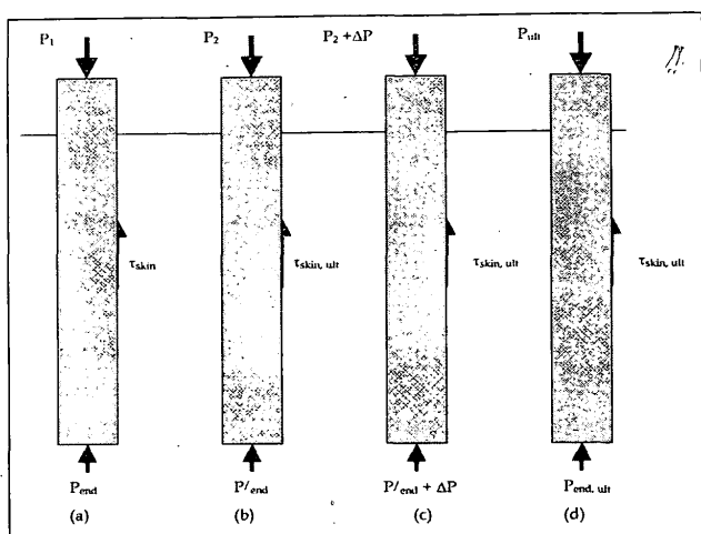
Figure 1: Load carrying through: (a) stage I; (b) end of stage I; (c) stage II and (d) end of stage III
