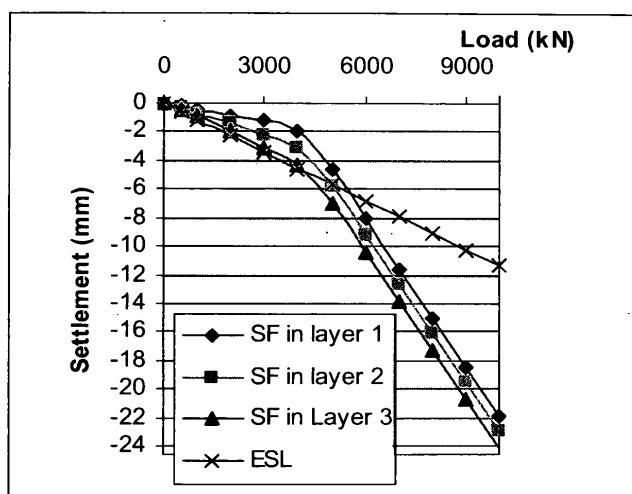
Figure 10: Effect of the location of the SF on the load-settlement curve baseline material parameters (End quake 10 mm).
