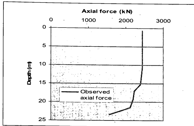
Figure 15: Measured axial force along the pile shaft (Hussein and Camp [2])
