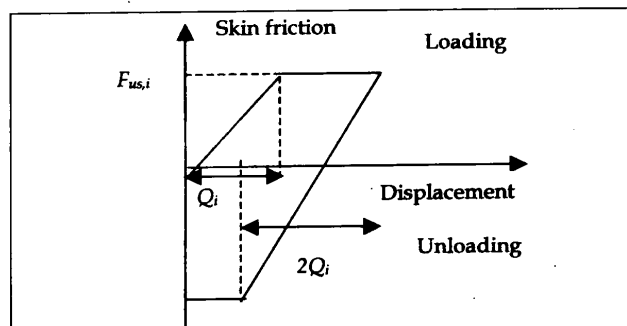
Figure 6: Load deflection behavior of a spring used to model the skin friction on i^{\text{th}} element.
