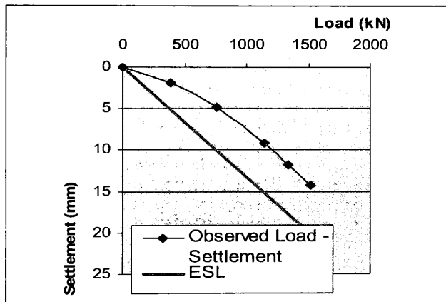
Figure 16: Load -settlement curve (Hussein and Camp [2])
