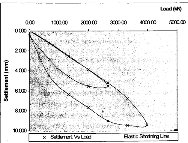
Figure 4: Category III - Initial portion of the load-settlement curve is below the ES
