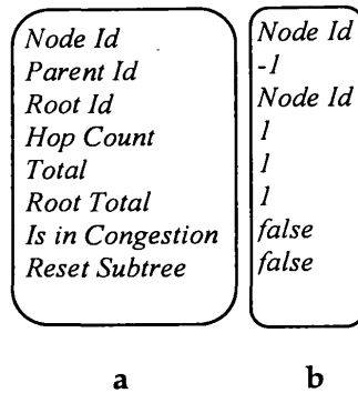
Figure 2 - (a) Beacon packet structure. (b) Default values of the beacon
