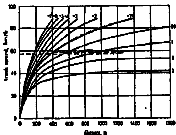
Performance Cures for 5 kW/Tonne Trucks on Downgrades
