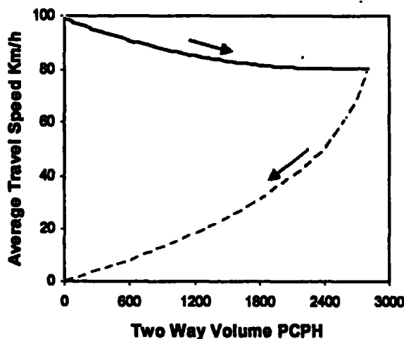
Figure 2. Relationship between Average Speed and Flow Rate
