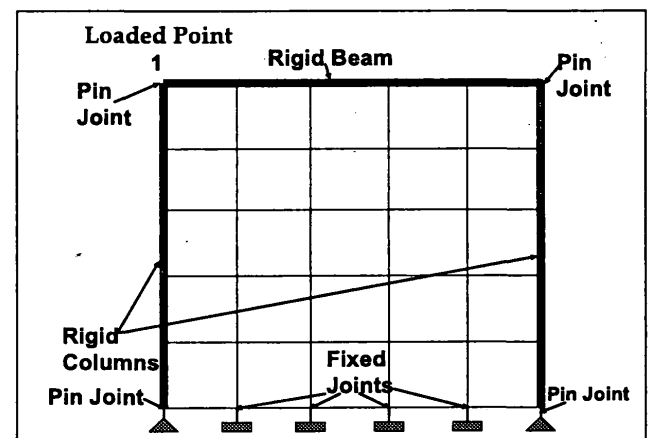
Figure 3: Two rigid columns and the rigid beam with the wall panel (Case 03)
