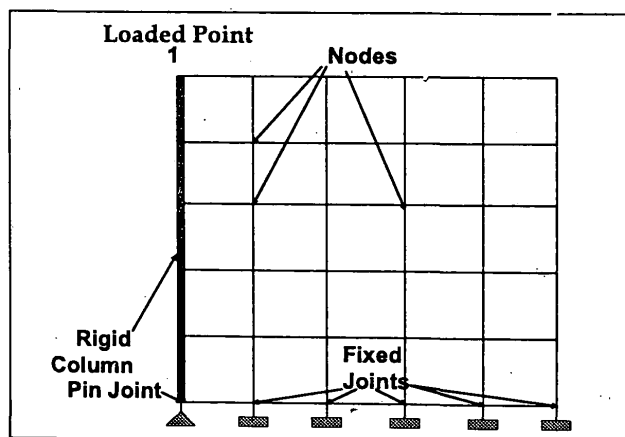
Figure 1. Rigid column with the wall panel (Case 01)
