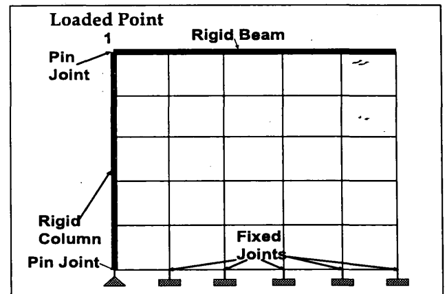
Figure 2: Rigid column and the rigid beam with the wall panel (Case 02)
