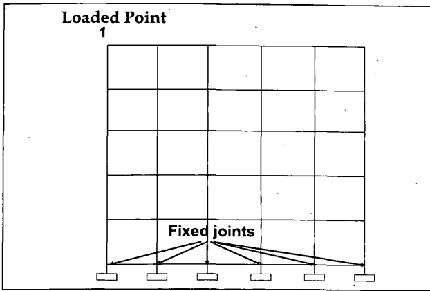
Figure 4: Without any rigid elements with the wall panel (Case 04)
