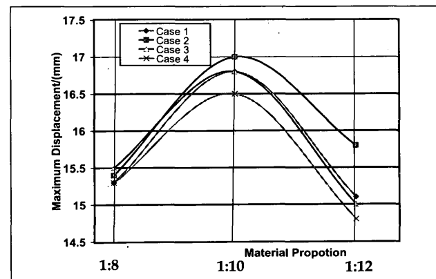
Figure 5: Maximum Displacements/ (mm) Vs Material Proportions
