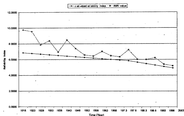
Figure 3 - Comparison of calculated and predicted Reliability Index for ANN training set
