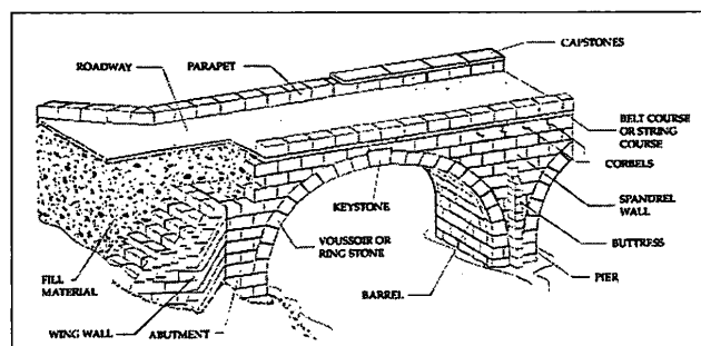
Figure 1 - Main parts of the masonry arch bridge
