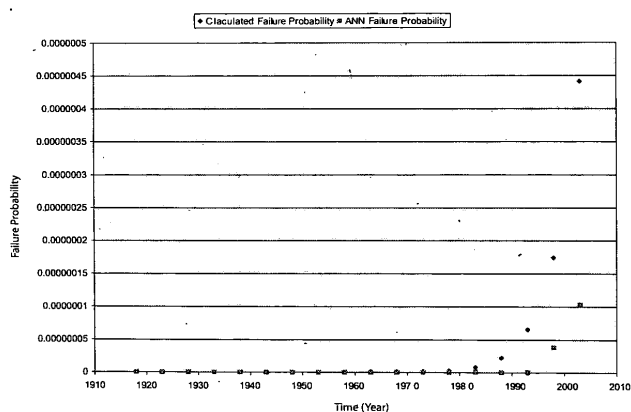
Figure 4 - Comparison of calculated and predicted Failure Probability for ANN training set
