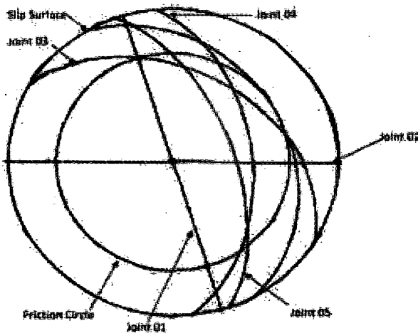
Figure 8 - Stereonet plot of great circles of rock discontinuities
