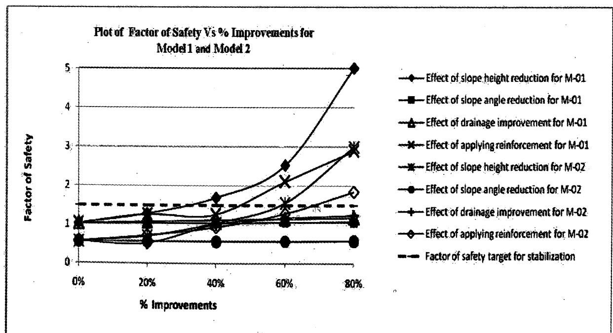
Figure 10 - Variation of Factor of Safety with Percentage improvement for both Failure Models
