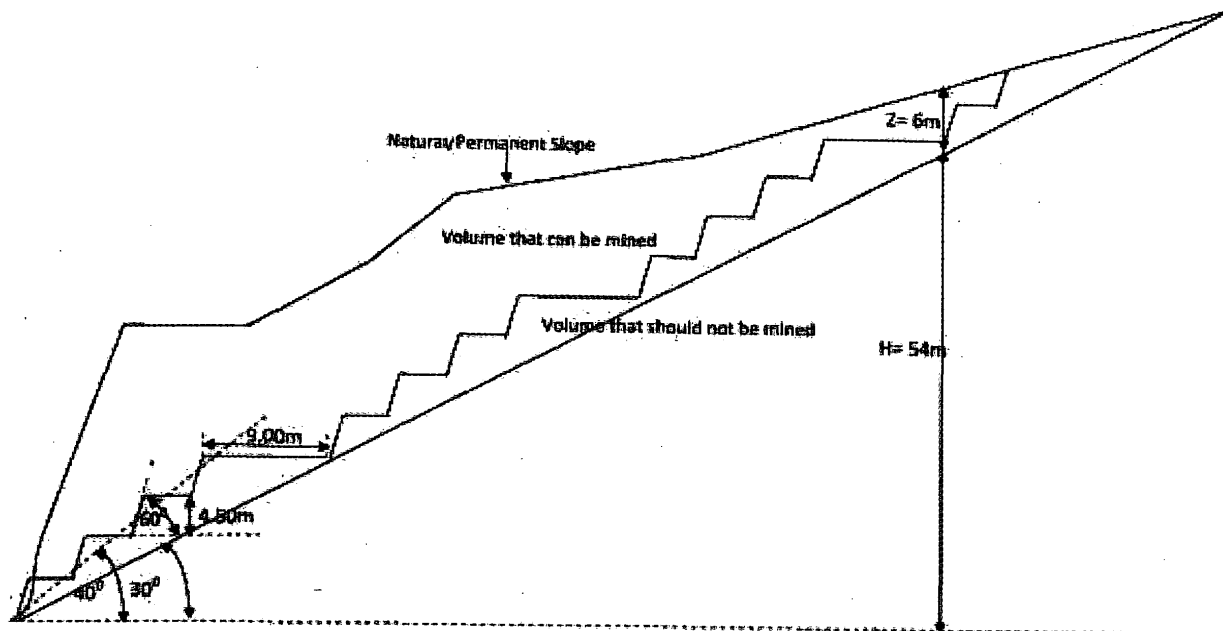
Figure 11 - Model Slope Design for failed slope
