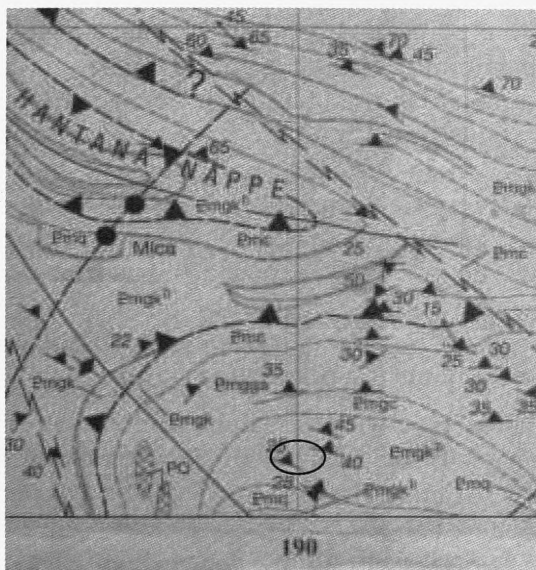
Figure 5 - Structural Geology of the area
