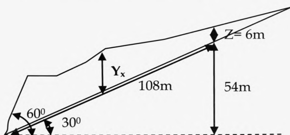
Figure 6 - Approximate Geometry of failed slope
