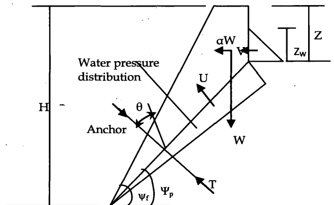
Figure 1 - Model 01: with a tension crack
