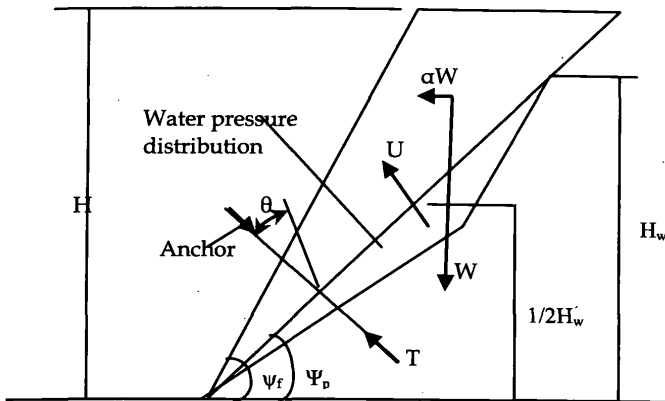
Figure 2 - Model 02: without a tension crack
