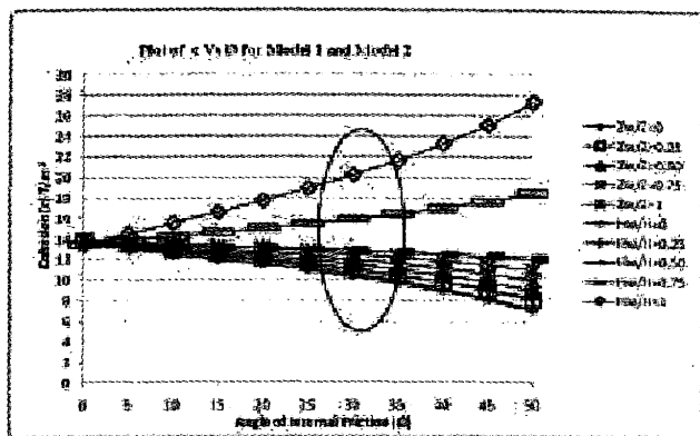
Figure 9 - Cohesion Vs Angle of Internal friction for both failure Models
