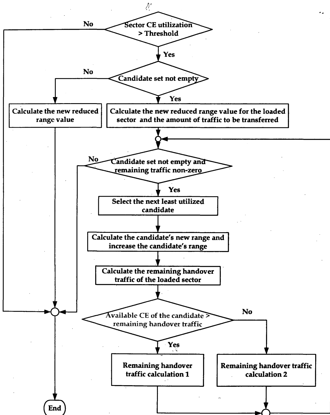
Figure 2 - Candidate BTS sector selection and range calculation
