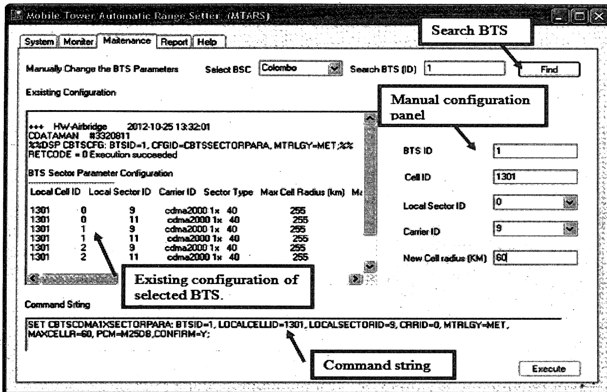
Figure 7 - Manual maintenance window
