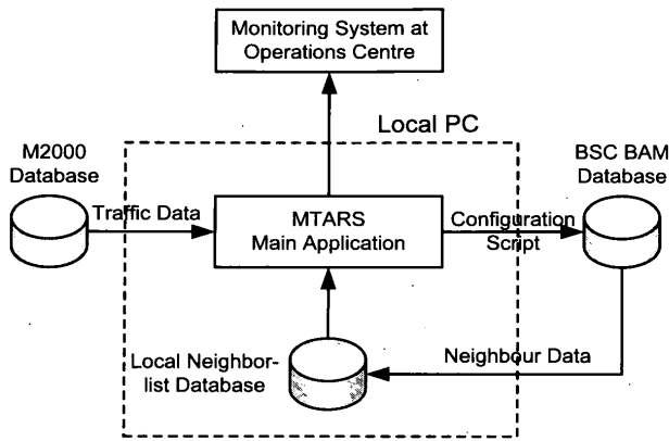
Figure 1- Proposed BTS sector range setter system architecture
