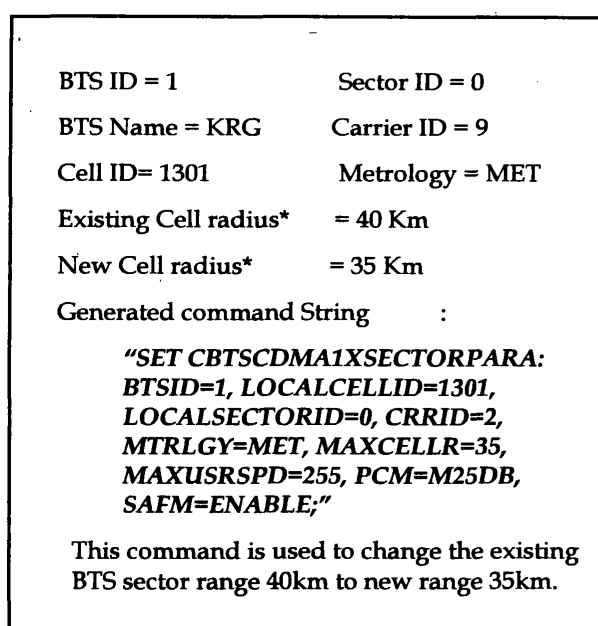
Figure 3 - Example CDMA2000 BSC command generation
