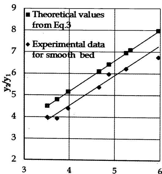
Figure 5- y_2/y_1 versus Froude Number
