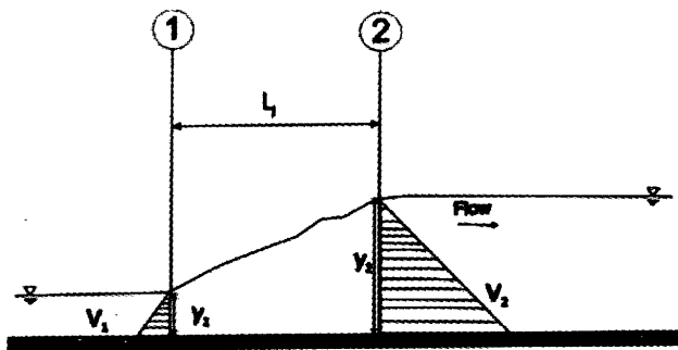
Figure 1 - Hydraulic Jump
