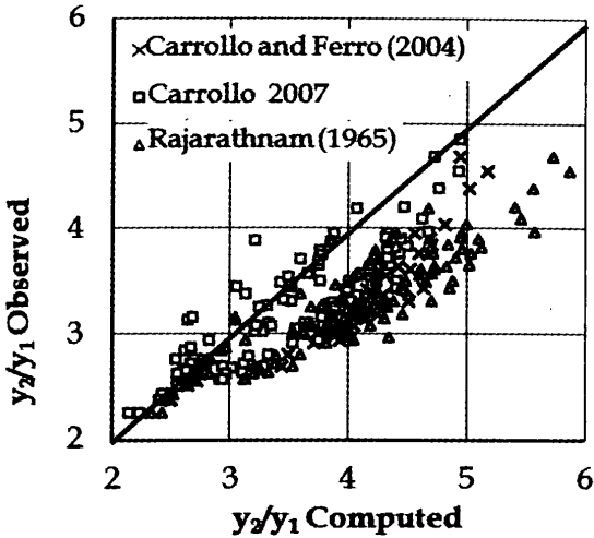
Figure 7 - y_2/y_1 observed vs. y_2/y_1 computed
