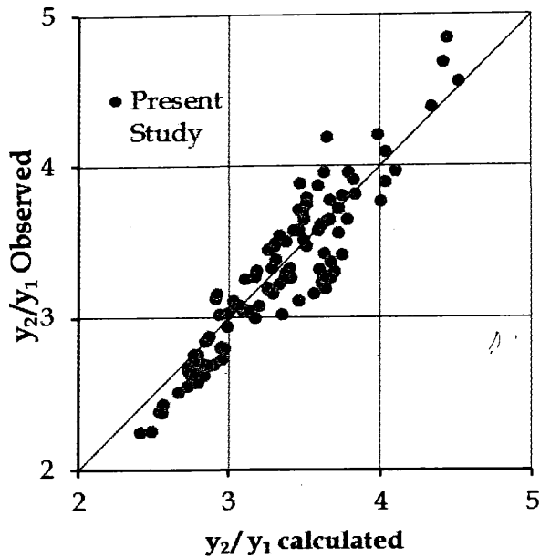
Figure 9- Prediction of y_2/y_1 for all the results using Eq. 11
