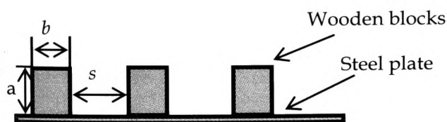
Figure 4- Arrangement of roughened bed
