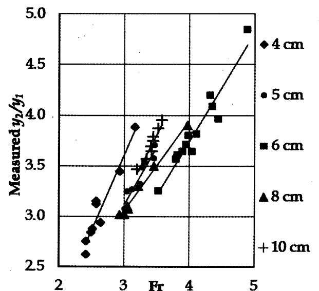
Figure 6- Measured y_2/y_1 versus Fr for 1.5 roughness elements for different spacing
