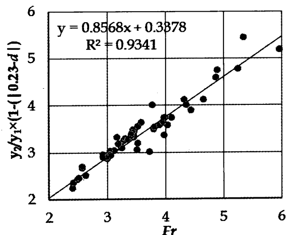
Figure 8- Relationship of d for 1.5 cm roughness element
